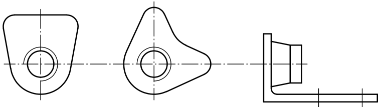
Figure 7 — Plate nuts, corner type
