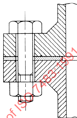
Figure 1 — Type A flange facings with full face gasket
