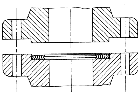
a) With sealing element only
