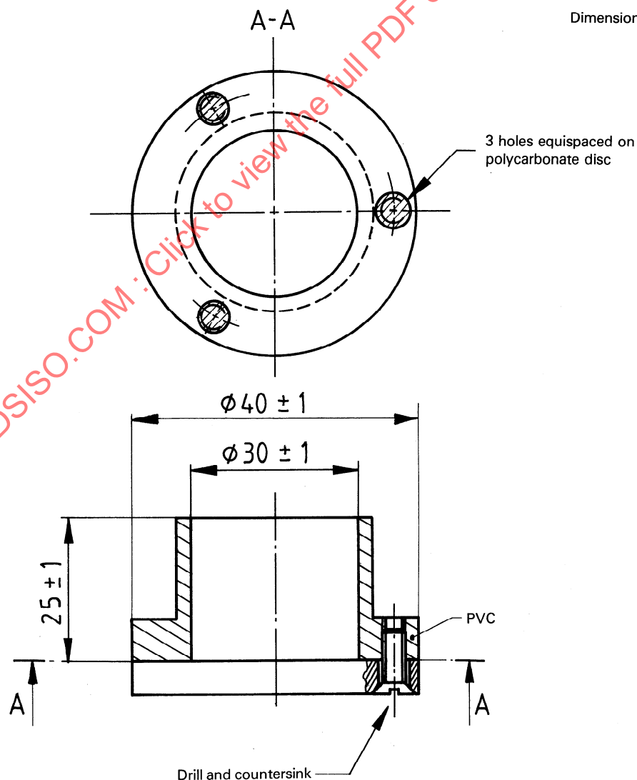
Figure 2 — Vicat test specimen holder
