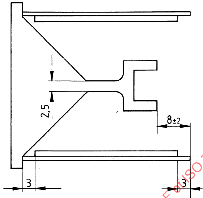
Figure 3 — Arrangement of mesio-occluso-distal inlay pattern and liner in casting ring
