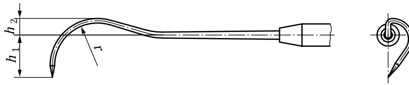
Figure 8 — Dental explorer
