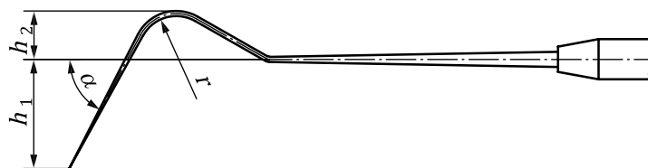
Figure 3 — Dental explorer
