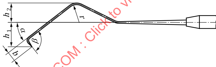
Figure 5 — Dental explorer
