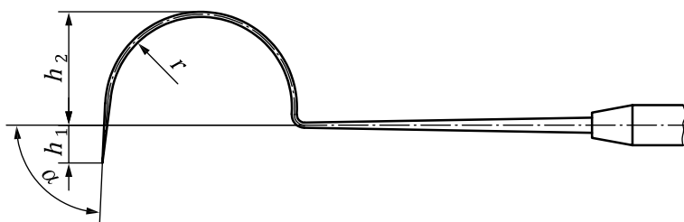
Figure 2 — Dental explorer
