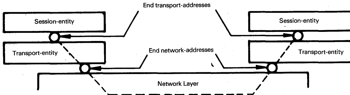
Figure 17 — Association of transport-addresses and network-addresses
