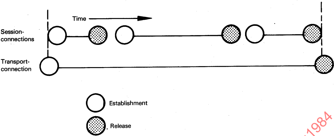
Figure 15 — Several consecutive session-connections
