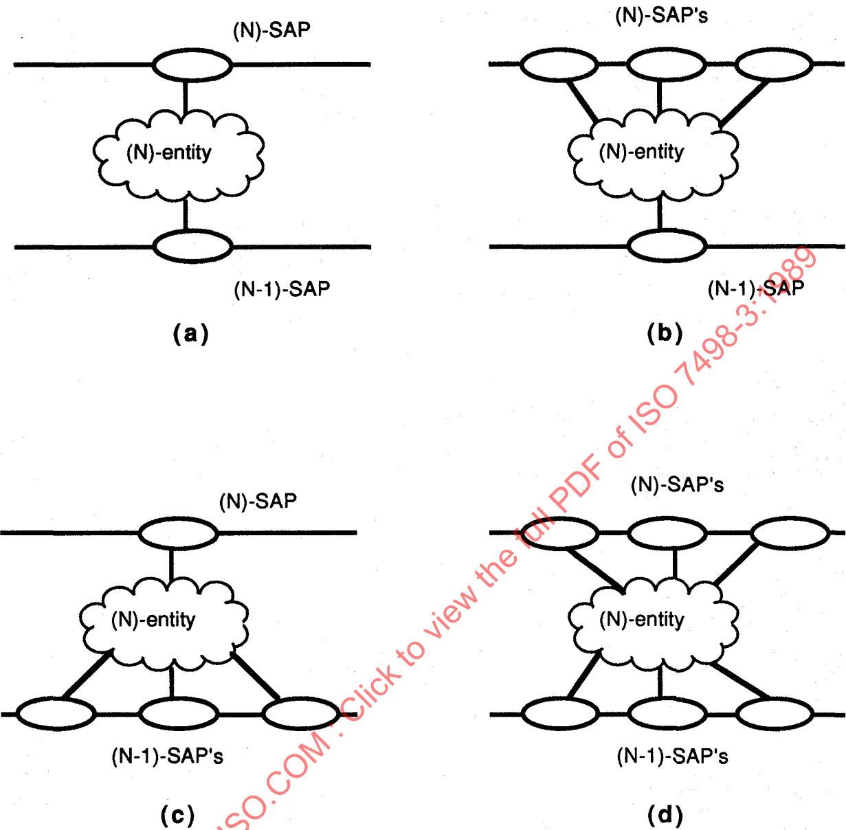
Figure 1 — Relationships of (N)-entity to (N)-SAPs and to (N-1)-SAPs
