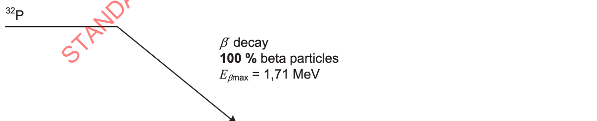
Figure B.2 — Decay scheme of ^{32}\text{P}
