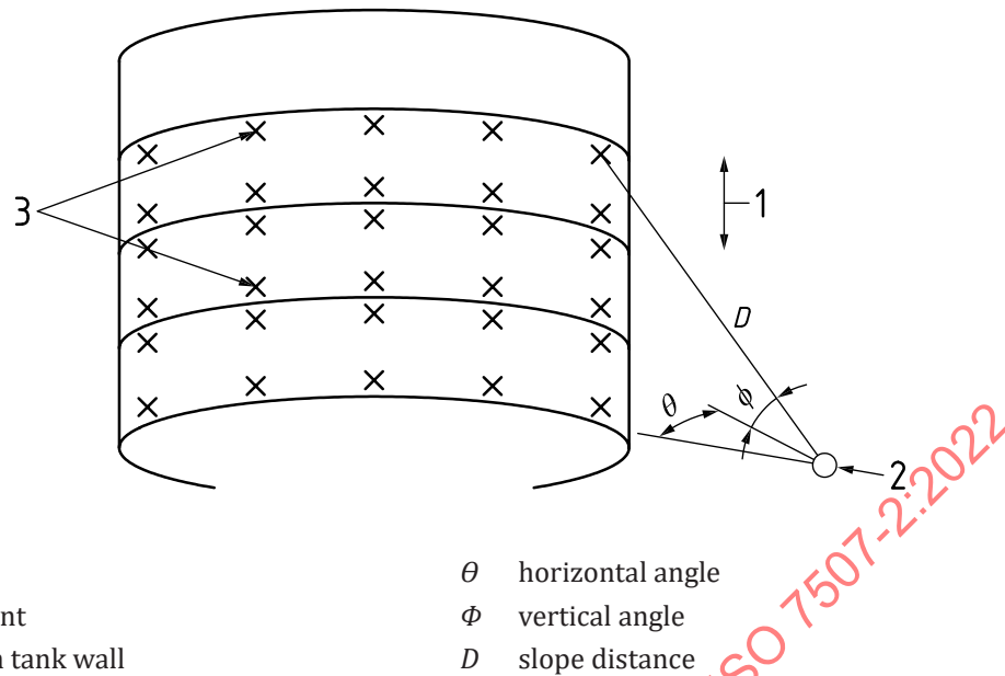
Figure 5 — Illustration of calibration procedure
