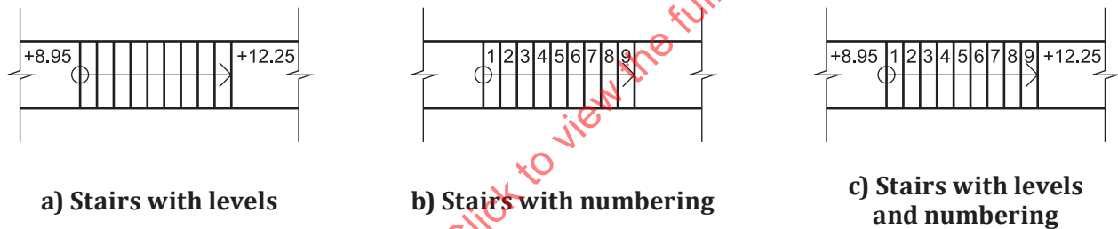
Figure 9 — Stairs with levels and step numbering
