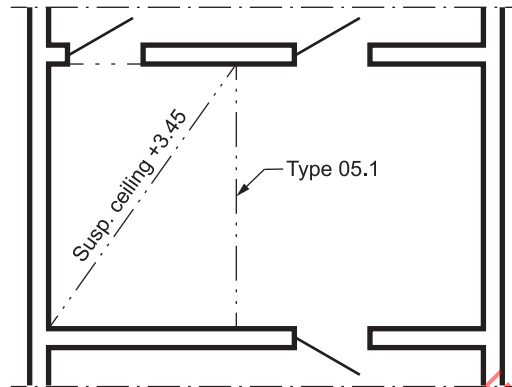
Figure 14 — Suspended ceiling
