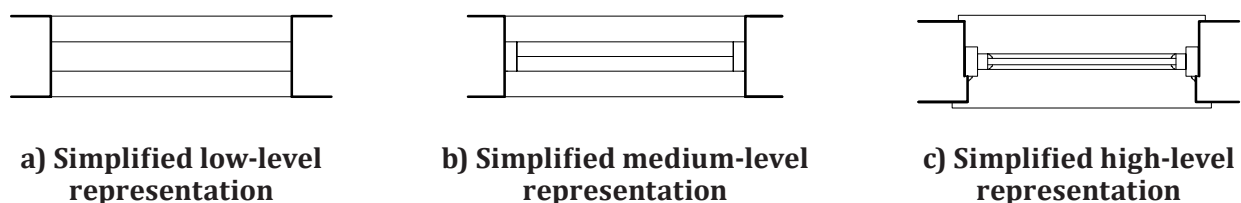
Figure 13 — Simplified representations for window in plan
