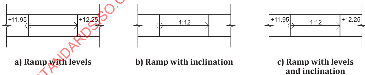
Figure 10 — Ramps with levels and inclination
