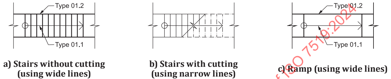
Figure 8 — Stairs and ramps
