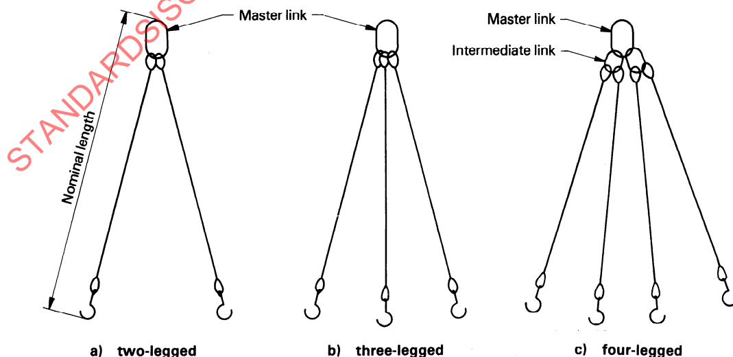
Figure 3 — Formation of typical sling assemblies
