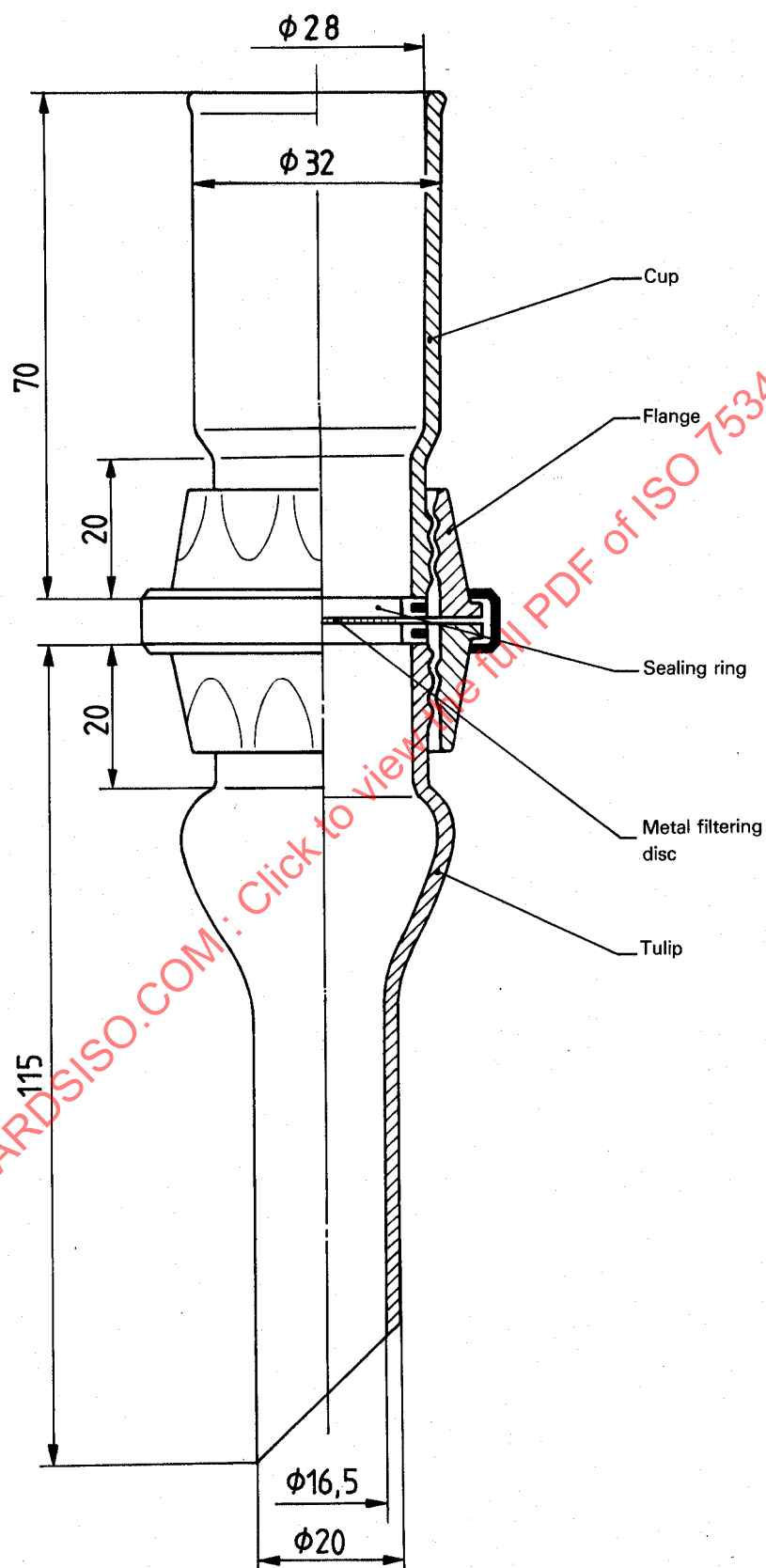
Figure — Filtration apparatus
