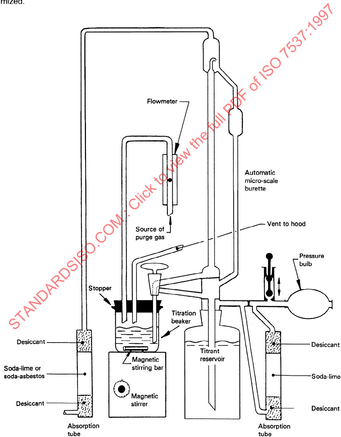
Figure 1 — Schematic drawing of typical apparatus
