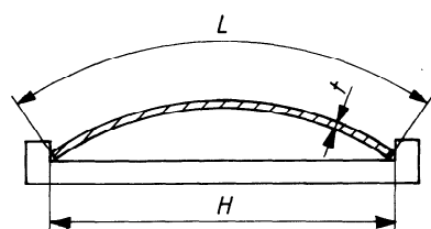
a) Two-point loaded specimen
