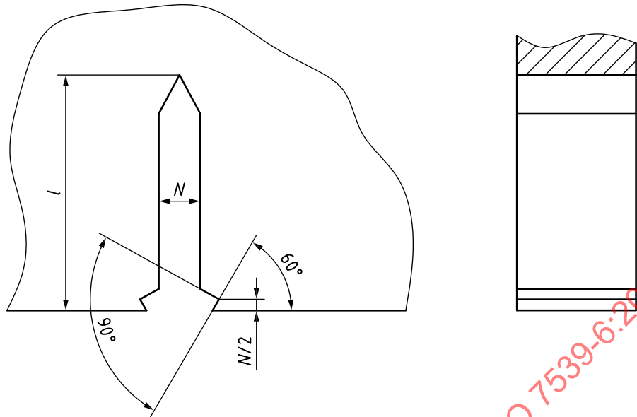
a) Integral type
