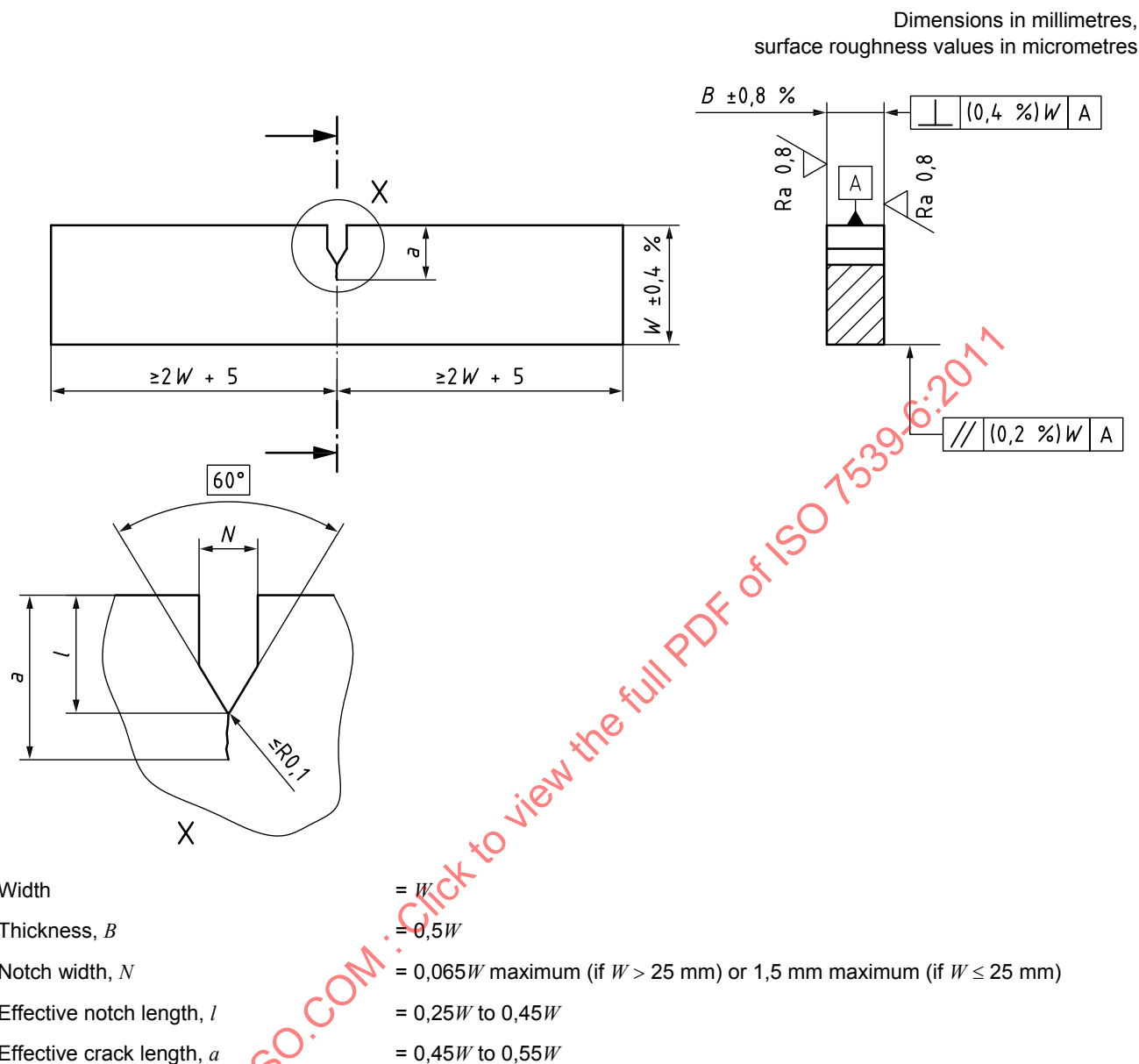
Figure 2 — Proportional dimensions and tolerances for cantilever bend test pieces
