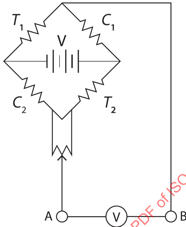
c) Bridge measurement circuit
