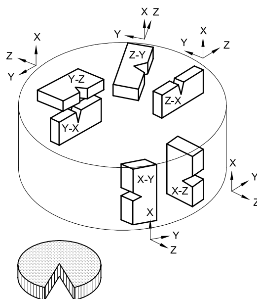
2) Axial grain flow — Radial working direction
