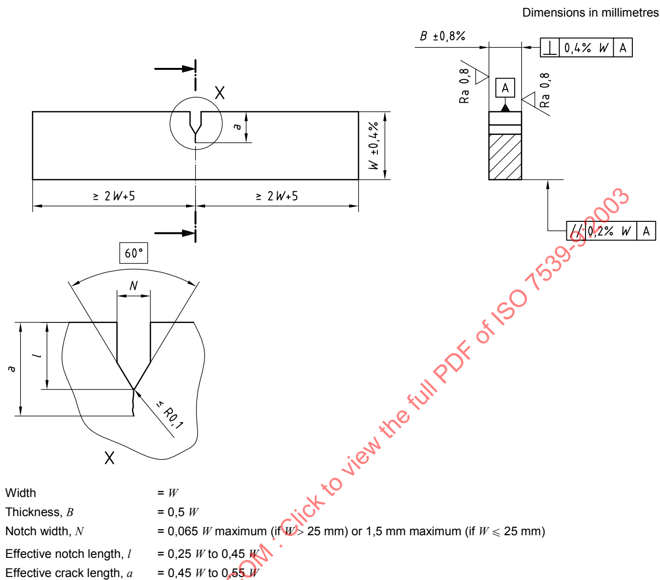
Figure 1 — Proportional dimensions and tolerances for cantilever bend test pieces
