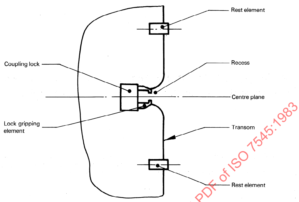
Figure 1 — Bow coupling of the pushboat/non-powered vessel
