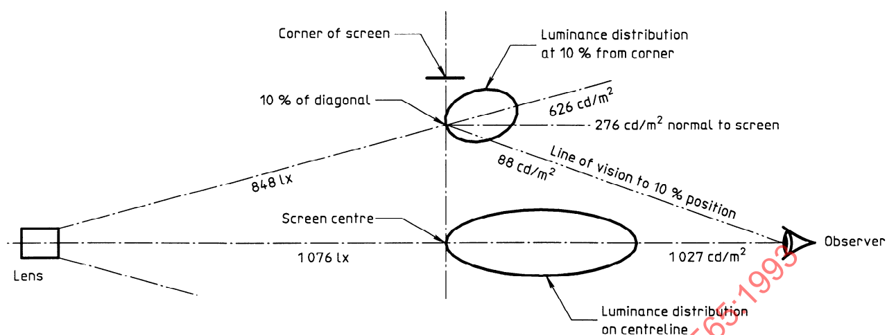
Figure A.1 — Effects of the actual scattering properties on viewing luminance
