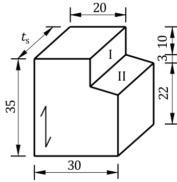
c) Test specimen for the bamboo strip (unit: mm)
