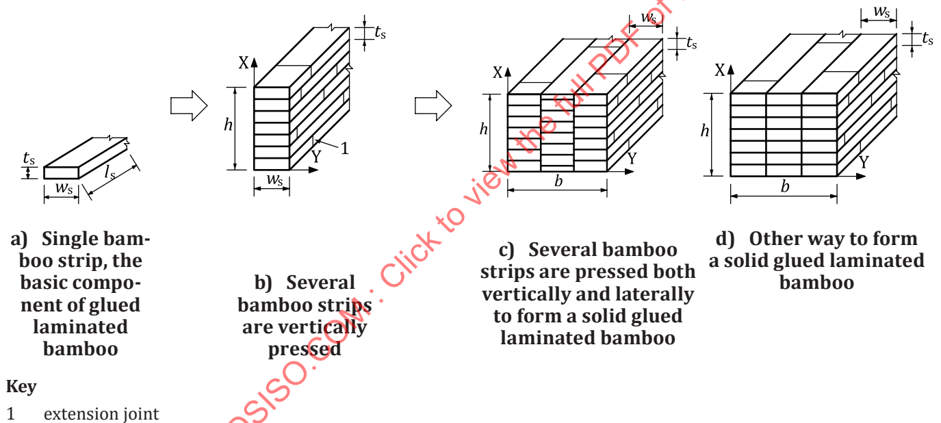
Figure 1 — Key manufacturing process for the products covered by this document
