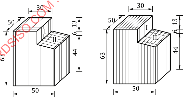
b) Test specimen for glued laminated bamboo (unit: mm)
