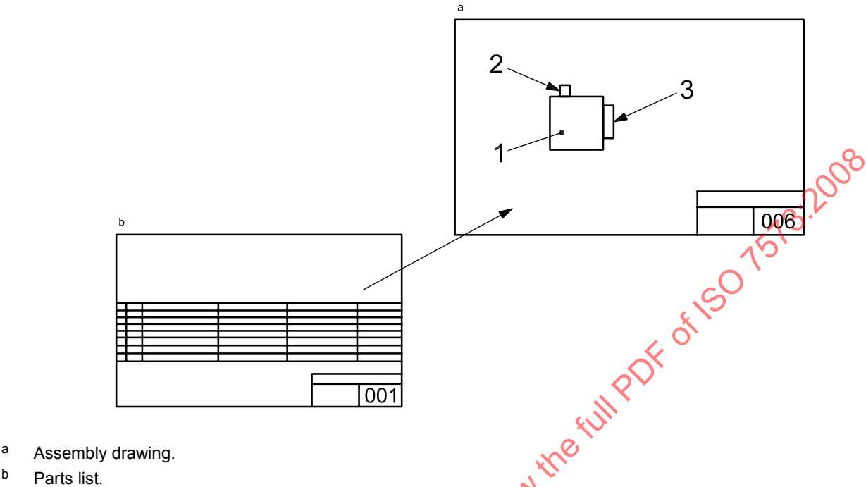
Figure A.3 — Parts list and assembly drawing as separate documents
