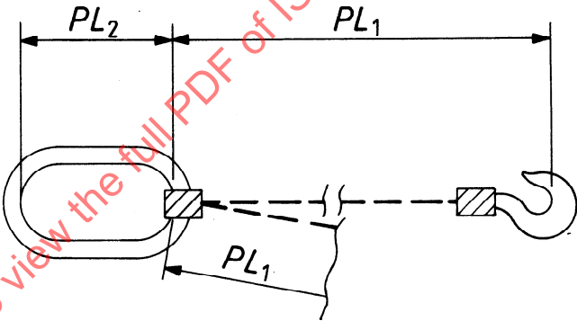
b) Double-branch sling
