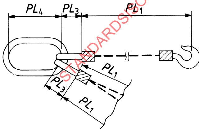
c) Three-branch sling
