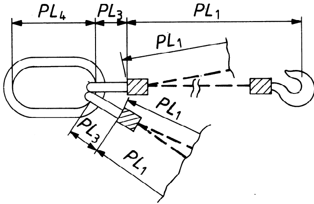
d) Four-branch sling
