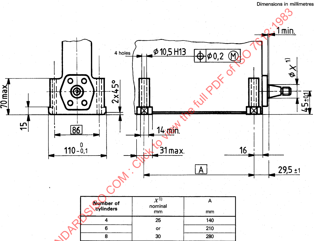
Figure 1 — Base mounted in-line fuel injection pump — Type 1
