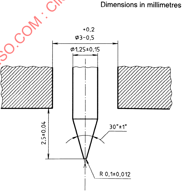
Figure 2 — Indentor for type D durometer
