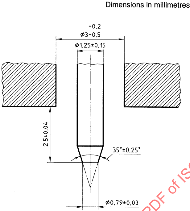
Figure 1 — Indentor for type A durometer
