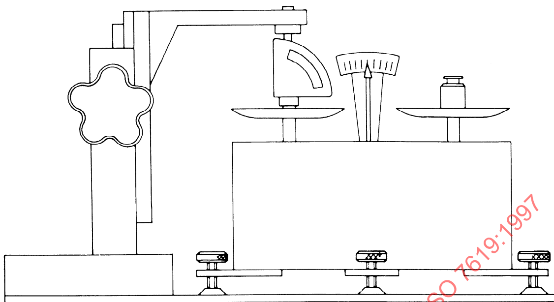
Figure 3 — Apparatus for calibration of durometer spring
