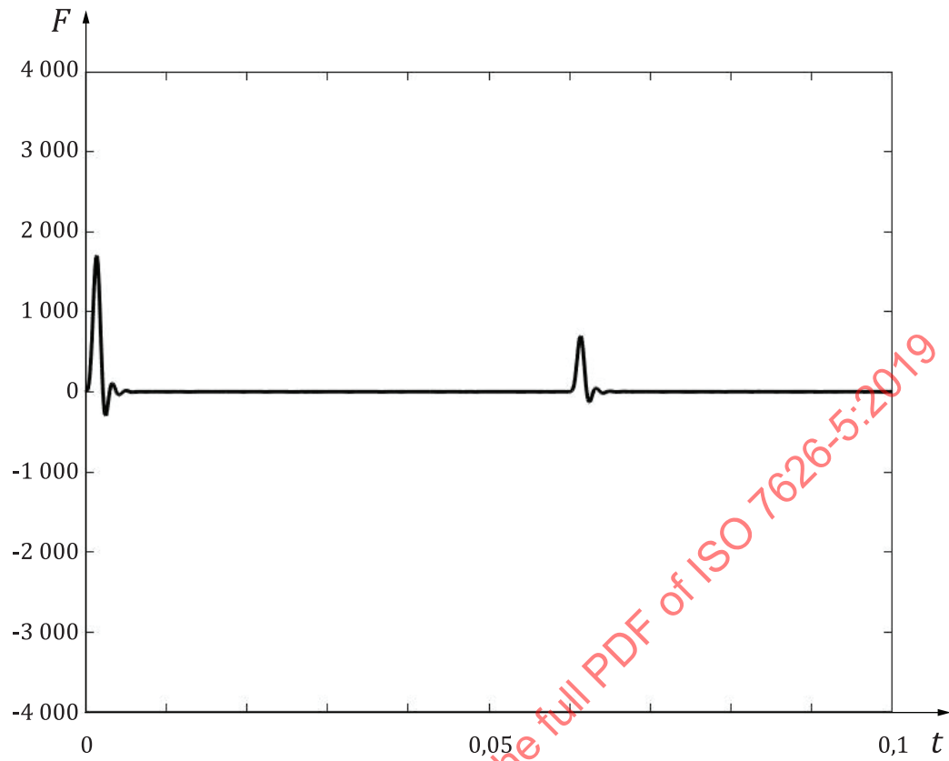
a) Time history of double-impact force
