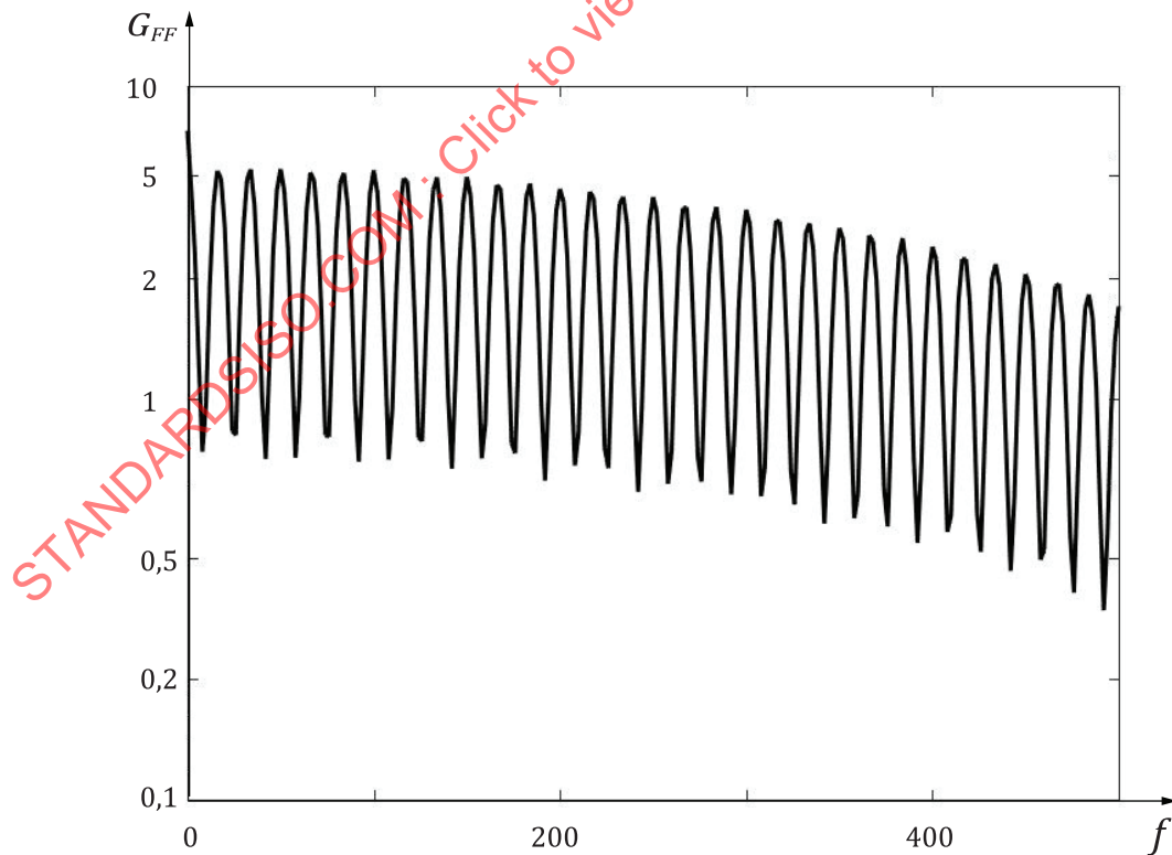
b) Energy spectral density corresponding to Figure 5 a)
