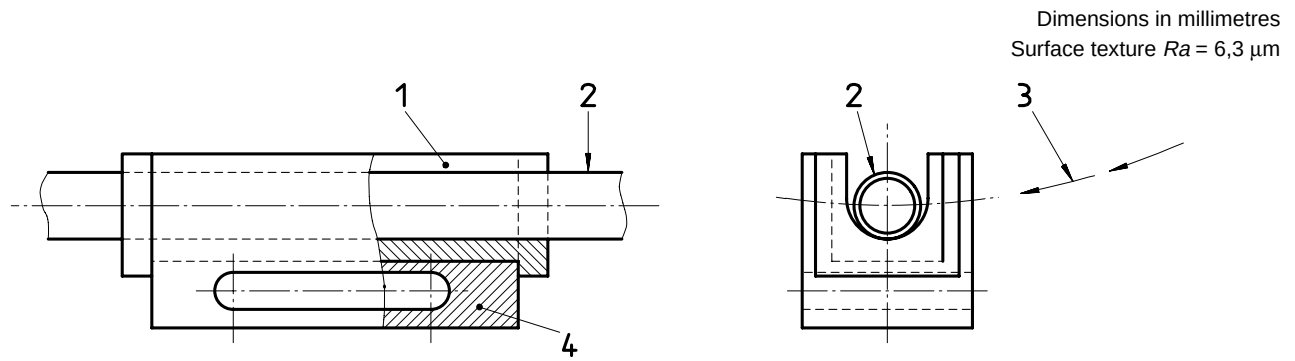
a) Assembled support showing tube sample in position
