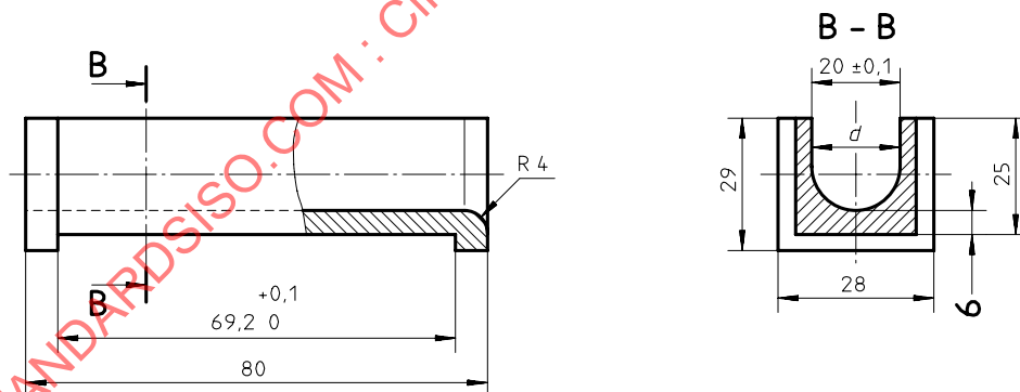
c) Part 2 [material: polyamid (PA) unsaturated polyester (UP), epoxyplastic (EP)]
