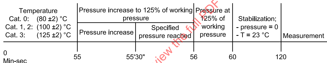
Figure 2 — Deformation under pressure; time line
