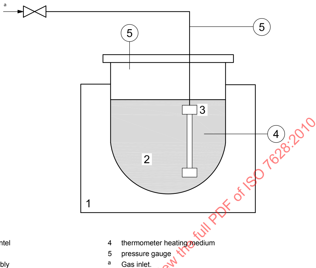
Figure 1 — Burst test at 125 °C — Schematic figure
