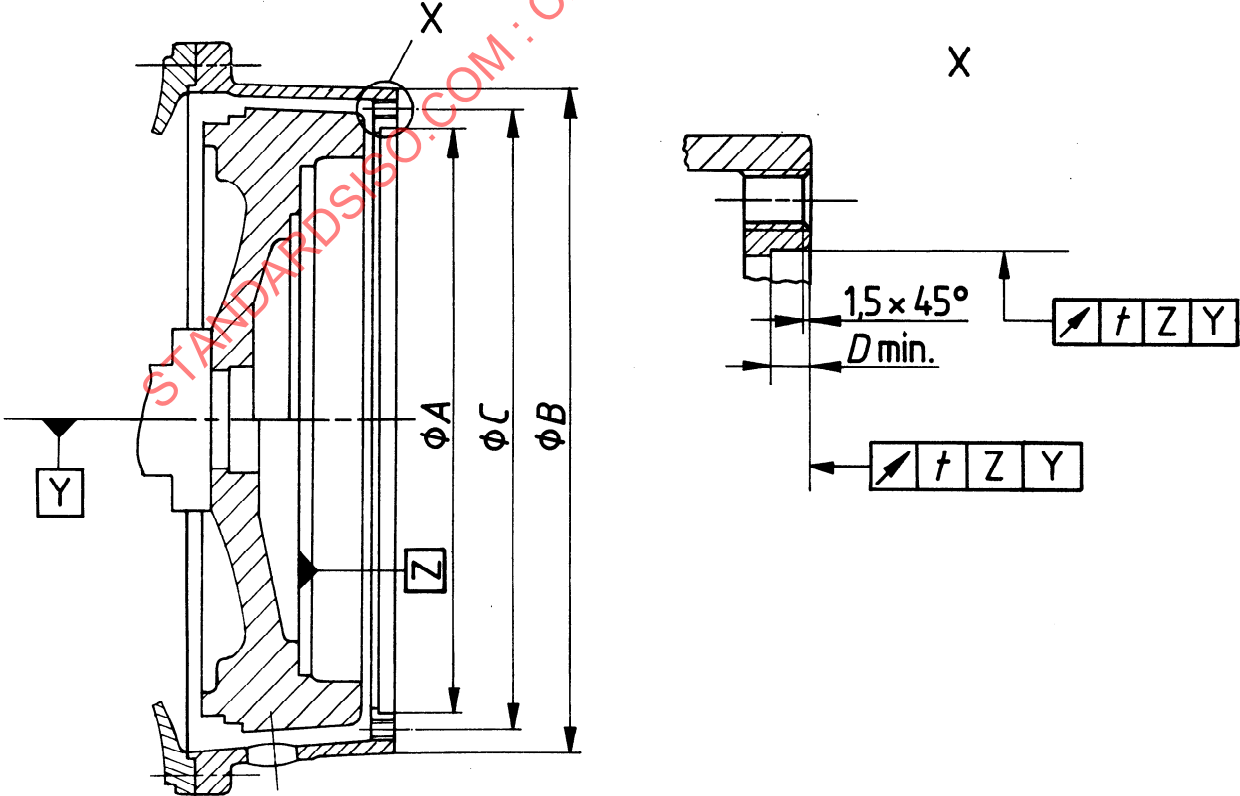
Figure 1 — Flywheel housing
