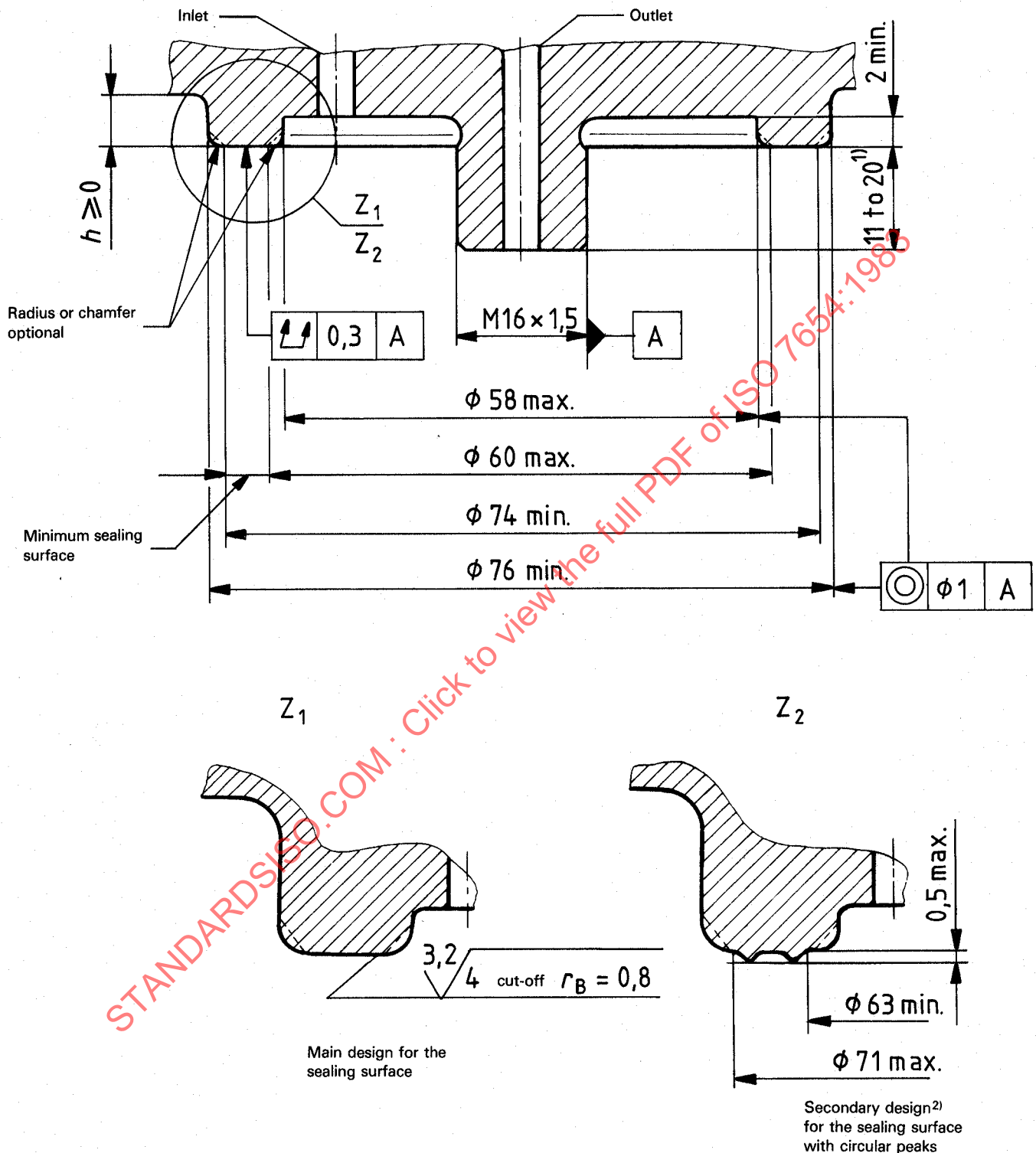
Figure 2 — Dimensions of sealing surface and connecting thread
