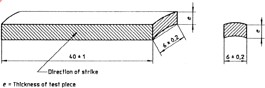
Figure D.1 — Test piece
