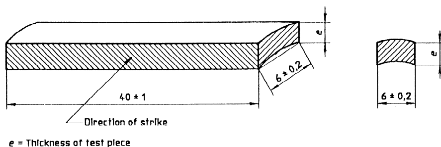
Figure D.1 — Test piece
