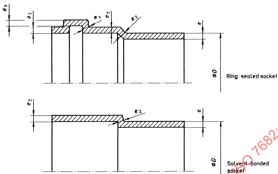
Figure 2 — Socket details
