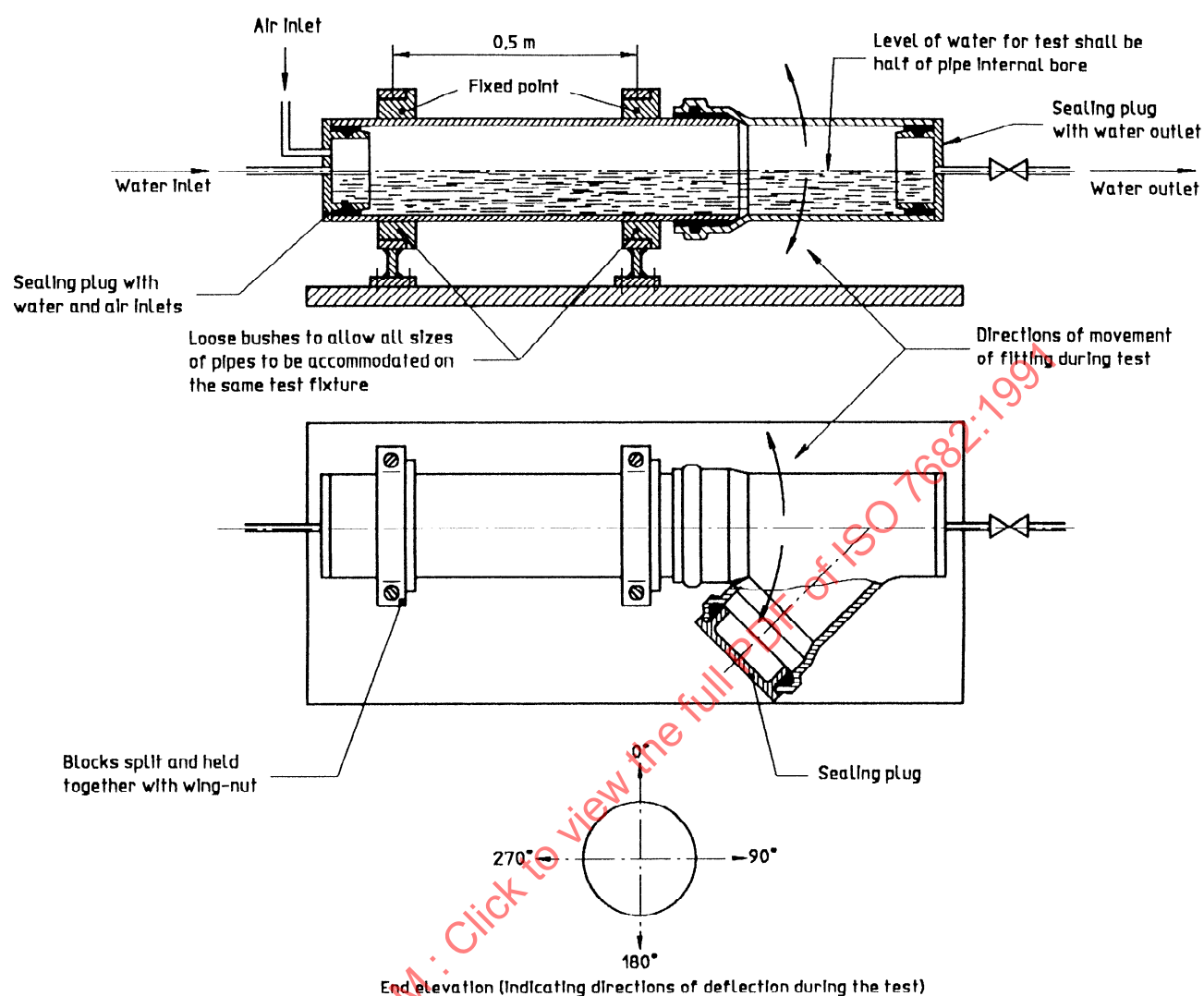
Figure G.1 — Test assembly for airtightness test
