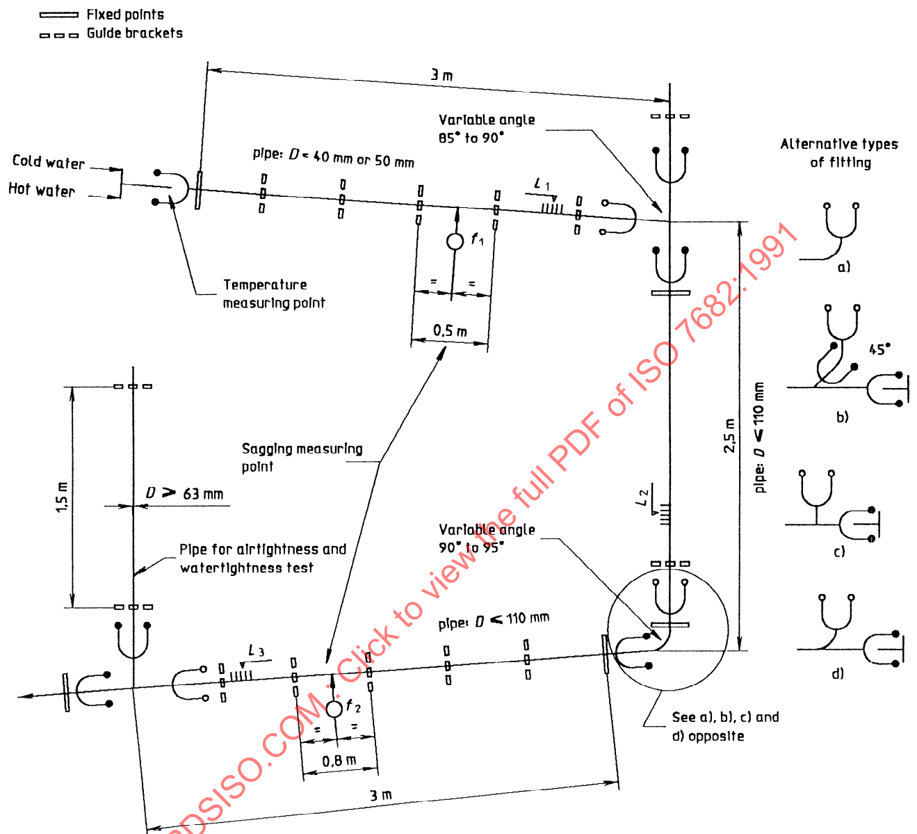
Figure J.1 — Test assembly for elevated-temperature cycling test (5 cycles)
