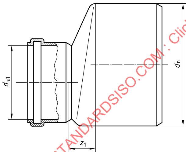
Figure 20 — Reducer
