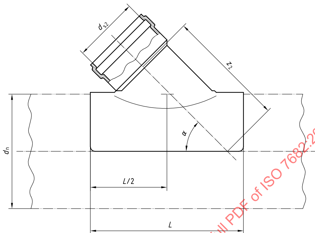
Figure 19 — Saddle branch
