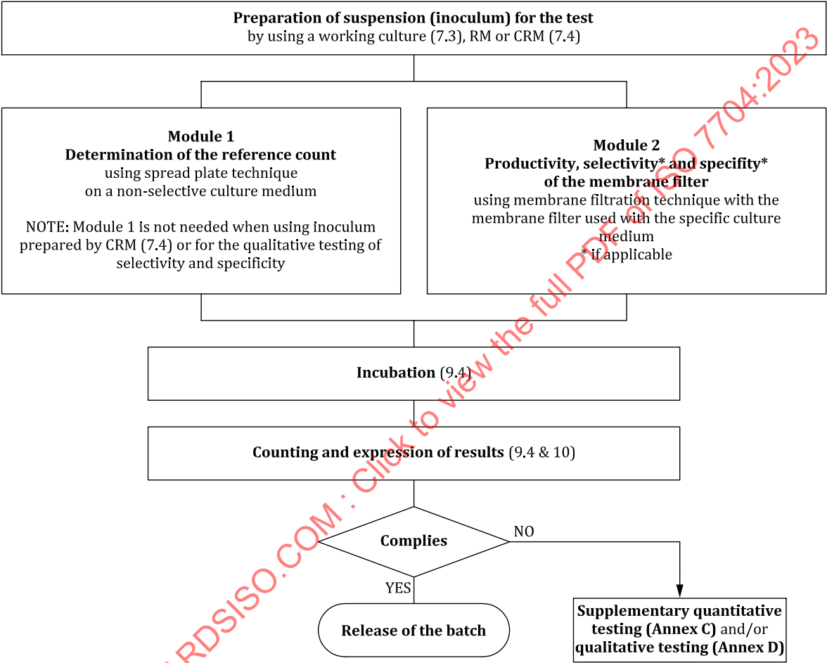
Figure A.1 — Diagram of the procedure for the batch testing
