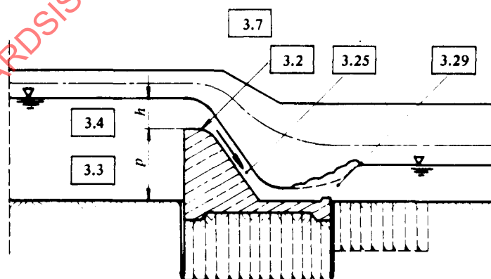
FIGURE 14 — Weir
