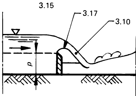
FIGURE 13 – Thin-plate weir
