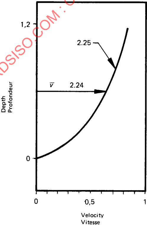
FIGURE 8 – Vertical velocity curve
