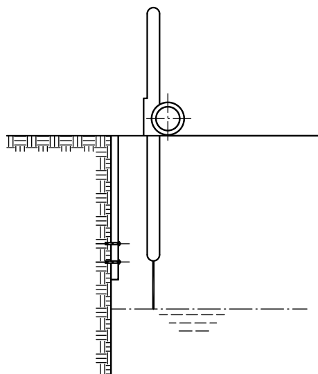
Figure 13 — Point gauge
