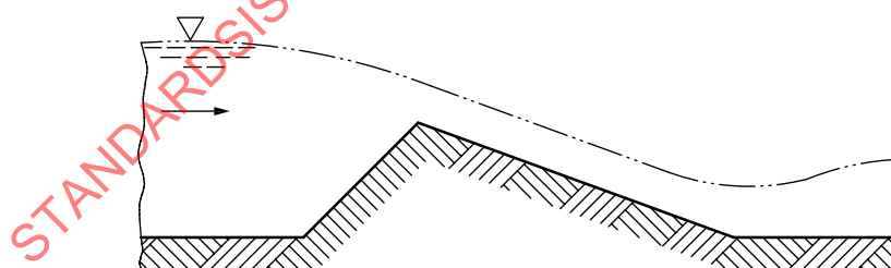
Figure 7 — Triangular-profile weir (longitudinal profile)
