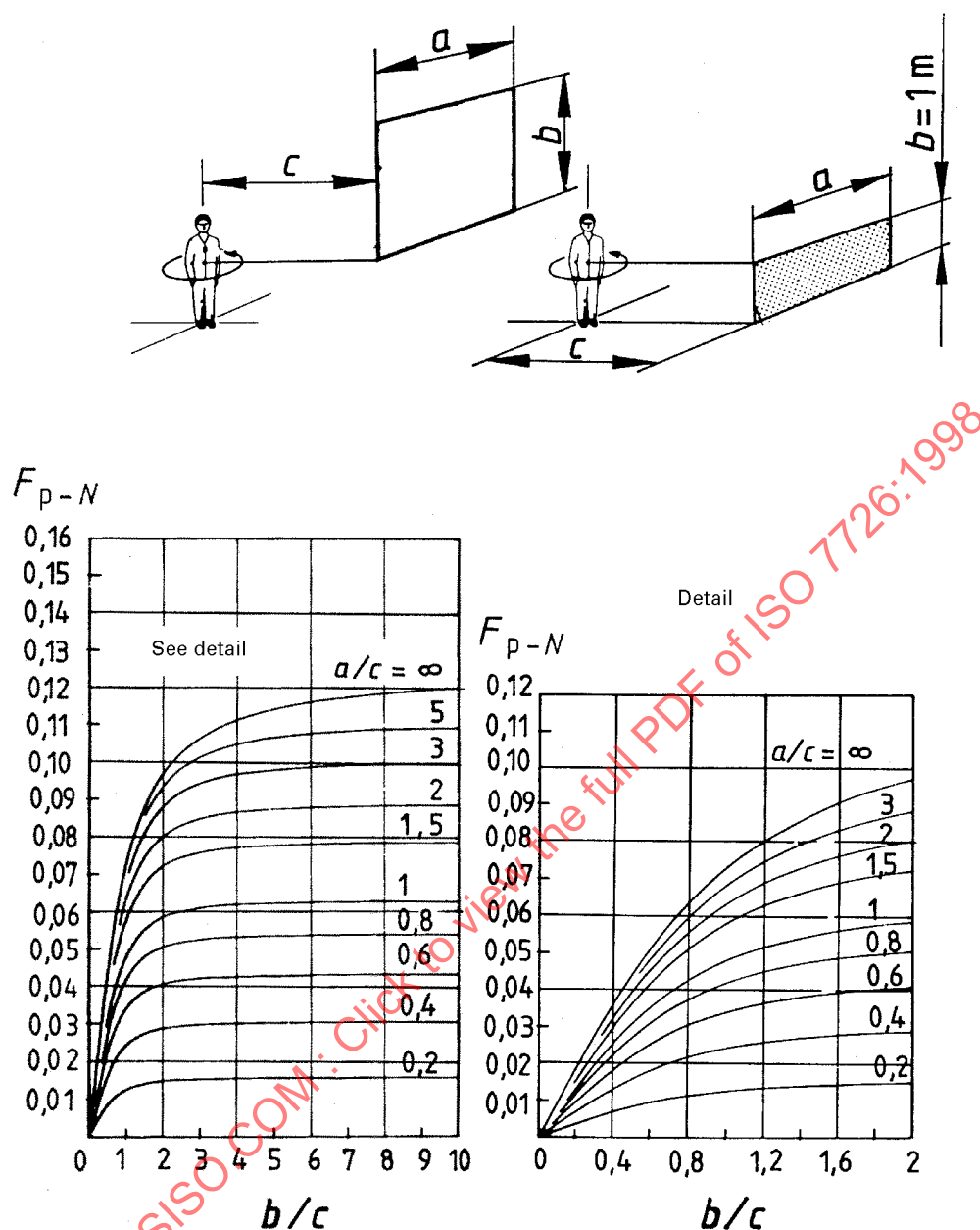
Figure B.4 — Mean value of angle factor between a standing person and a vertical rectangle (above or below his centre) when the person is rotated around a vertical axis. (To be used when the location but not the orientation of the person is known.)
