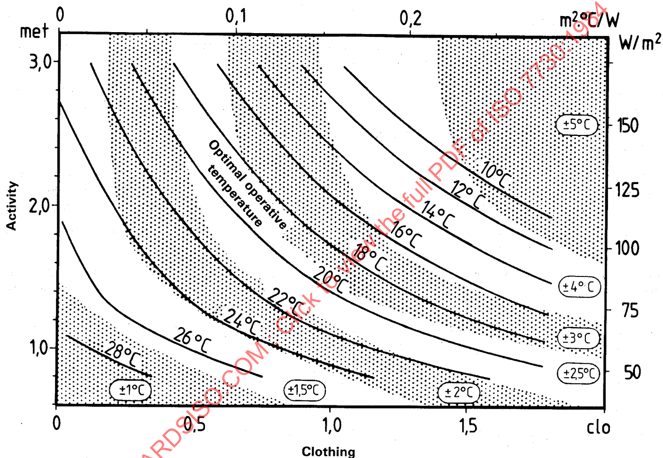
Figure 2 — The optimal operative temperature (corresponding to PMV = 0 ) as a function of activity and clothing
