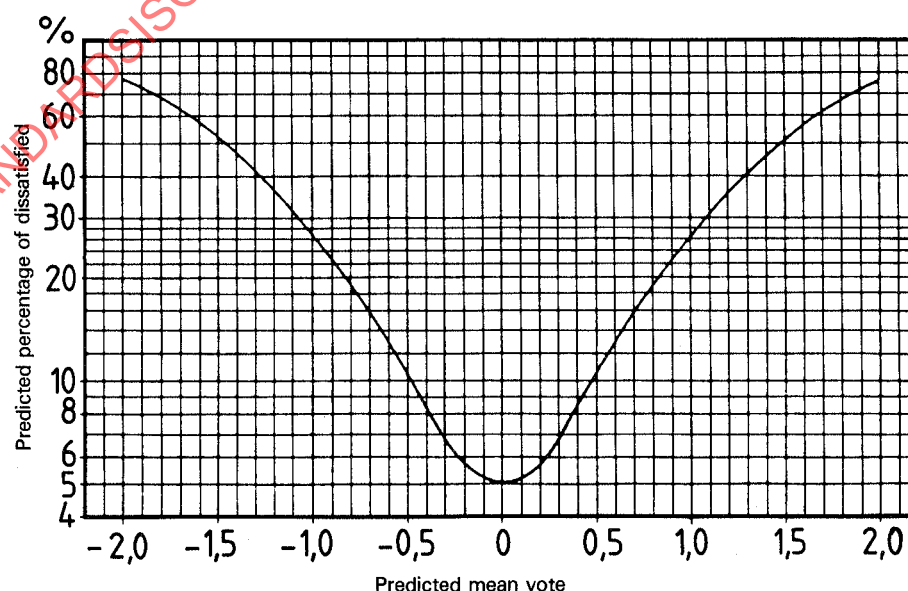
Figure 1 — Predicted percentage of dissatisfied (PPD) as a function of predicted mean vote (PMV)
