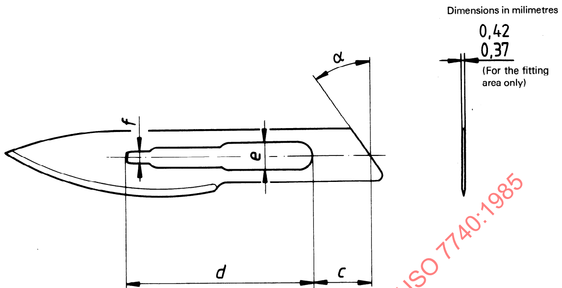
Figure 1 — Detachable blade
