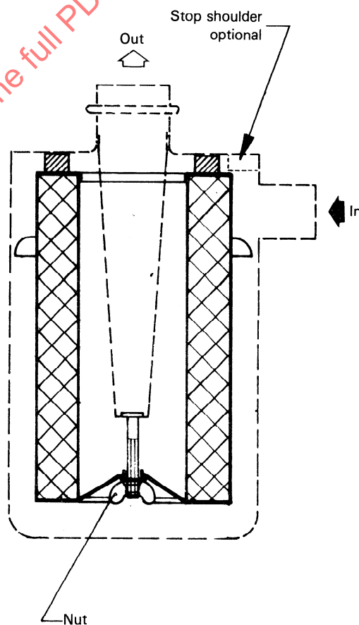
Figure 4 — Type C installation
