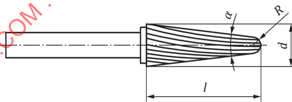
Figure 1 — Hardmetal burr, style L
