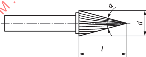
Figure 1 — Hardmetal burr, style M
