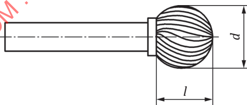
Figure 1 — Hardmetal burr, style D
