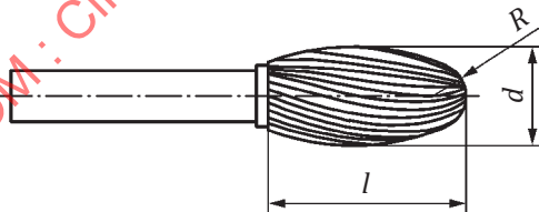
Figure 1 — Hardmetal burr, style E
