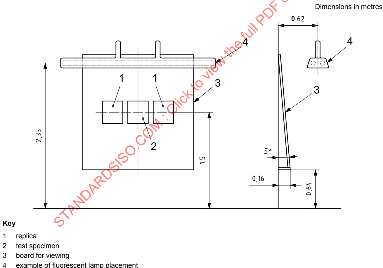
Figure 1 — Lighting equipment for viewing test specimens
