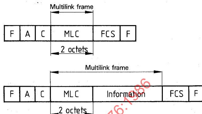
Figure 1 — Multilink frame formats
