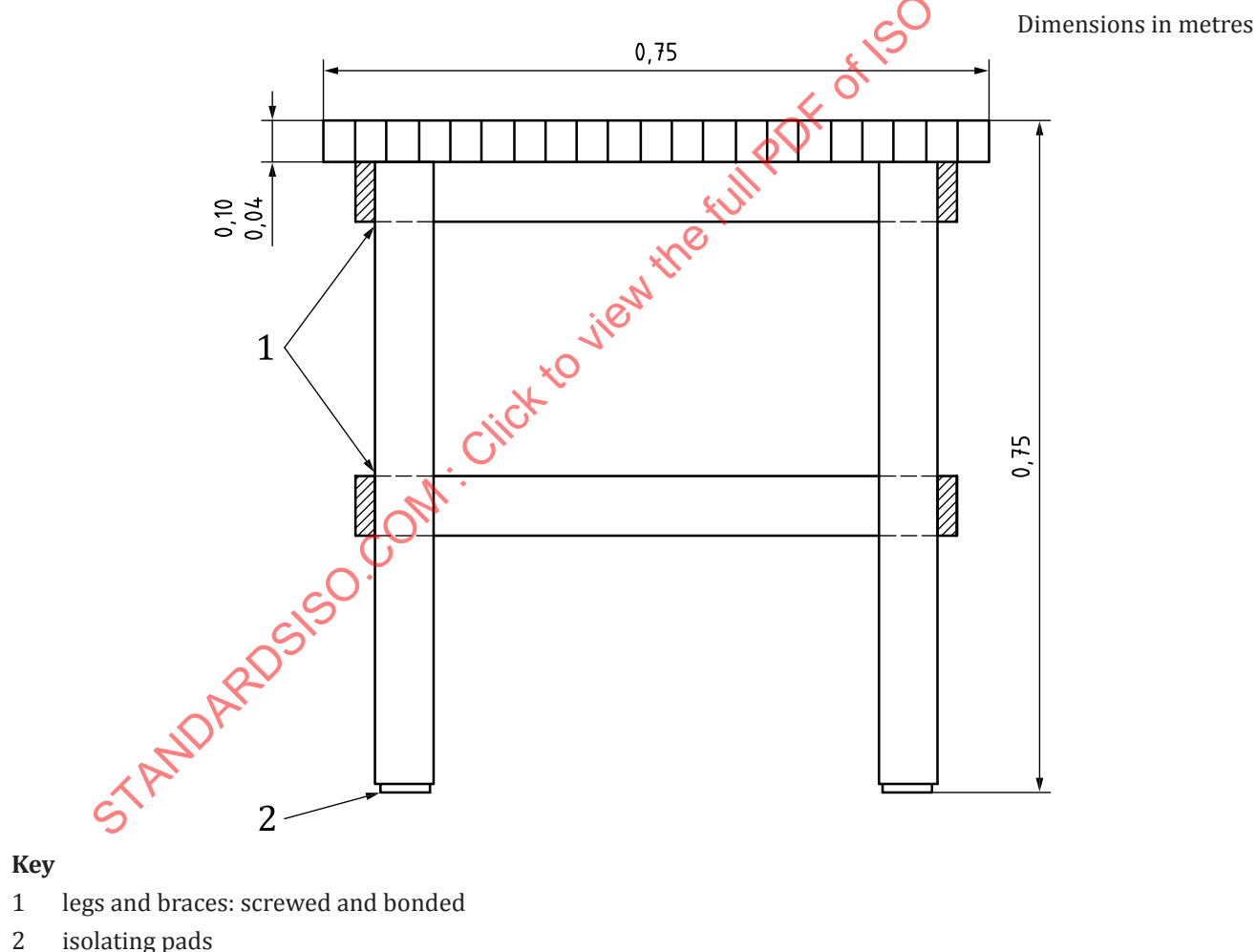
Figure A.1 — Standard test table
