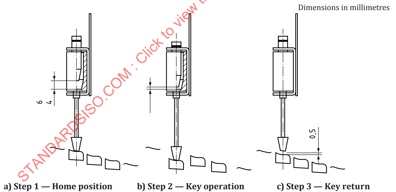
Figure A.4 — Individual steps of the solenoid operation
