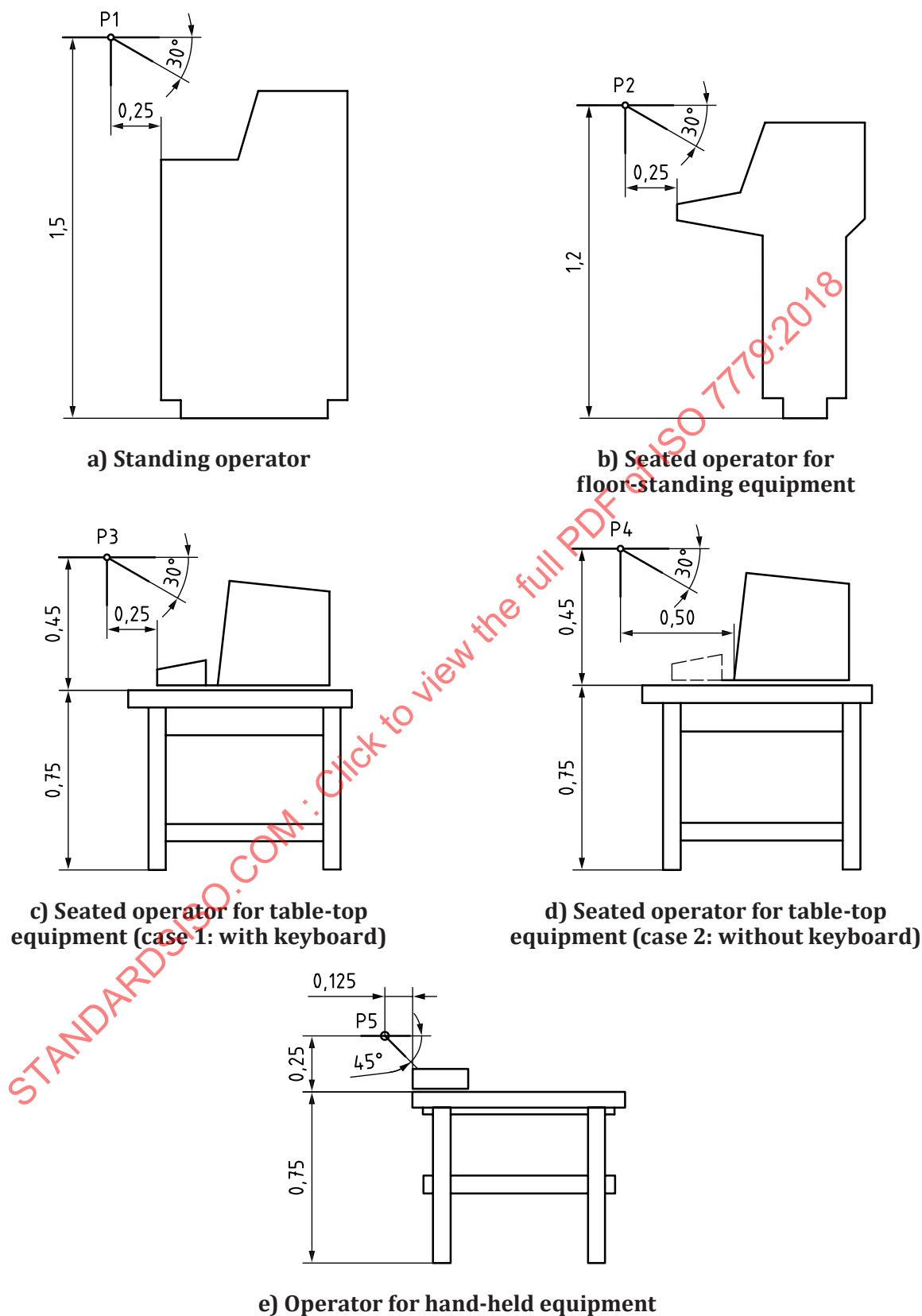
Figure 1 — Examples of microphone positions for standing and seated operators
