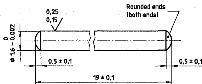
Figure 2 — Test mandrel
