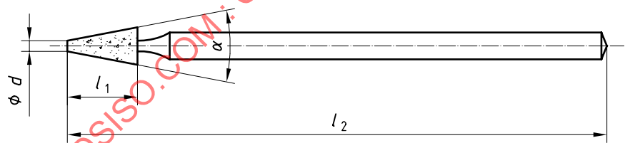
Figure 9 — Truncated conical, regular
