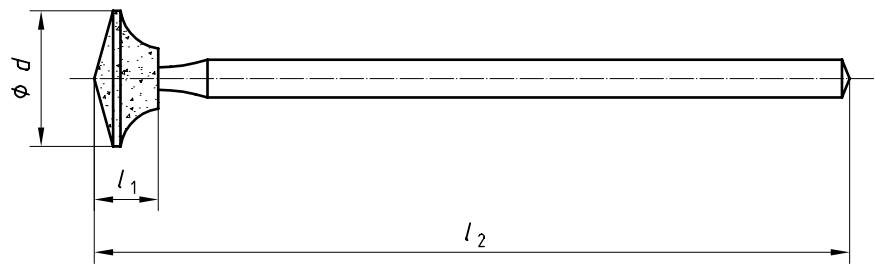
Figure 8 — Knife-edge (conico, inverted hyperboloidal)
