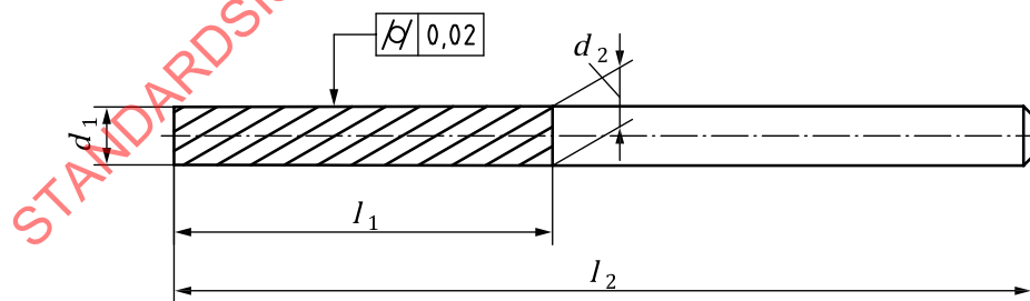
Figure 1 — Cylindrical, side cutting only
