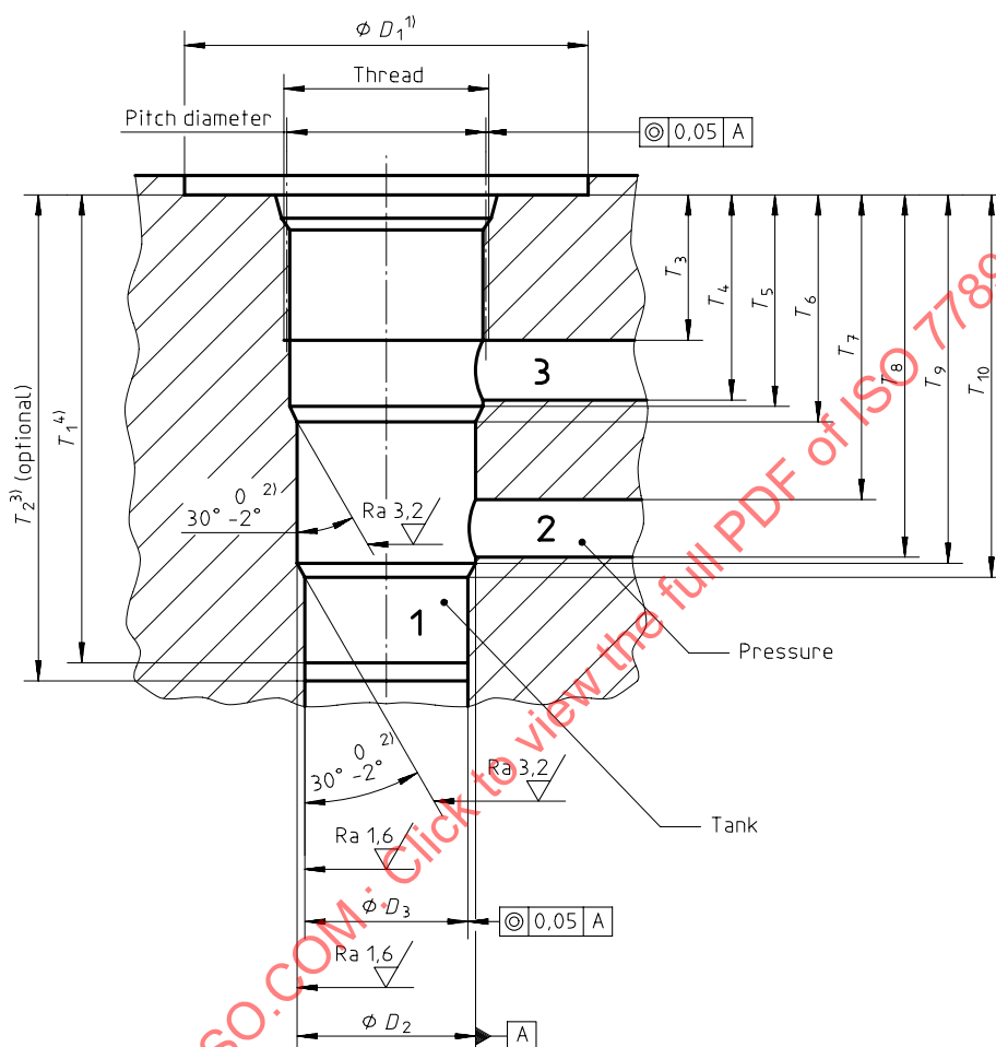
Figure 8 — Cavities for two-port main system pressure relief valves with 10,5 mm to 20,5 mm maximum main port diameter, one pilot port and flow direction from port 2 to port 1
