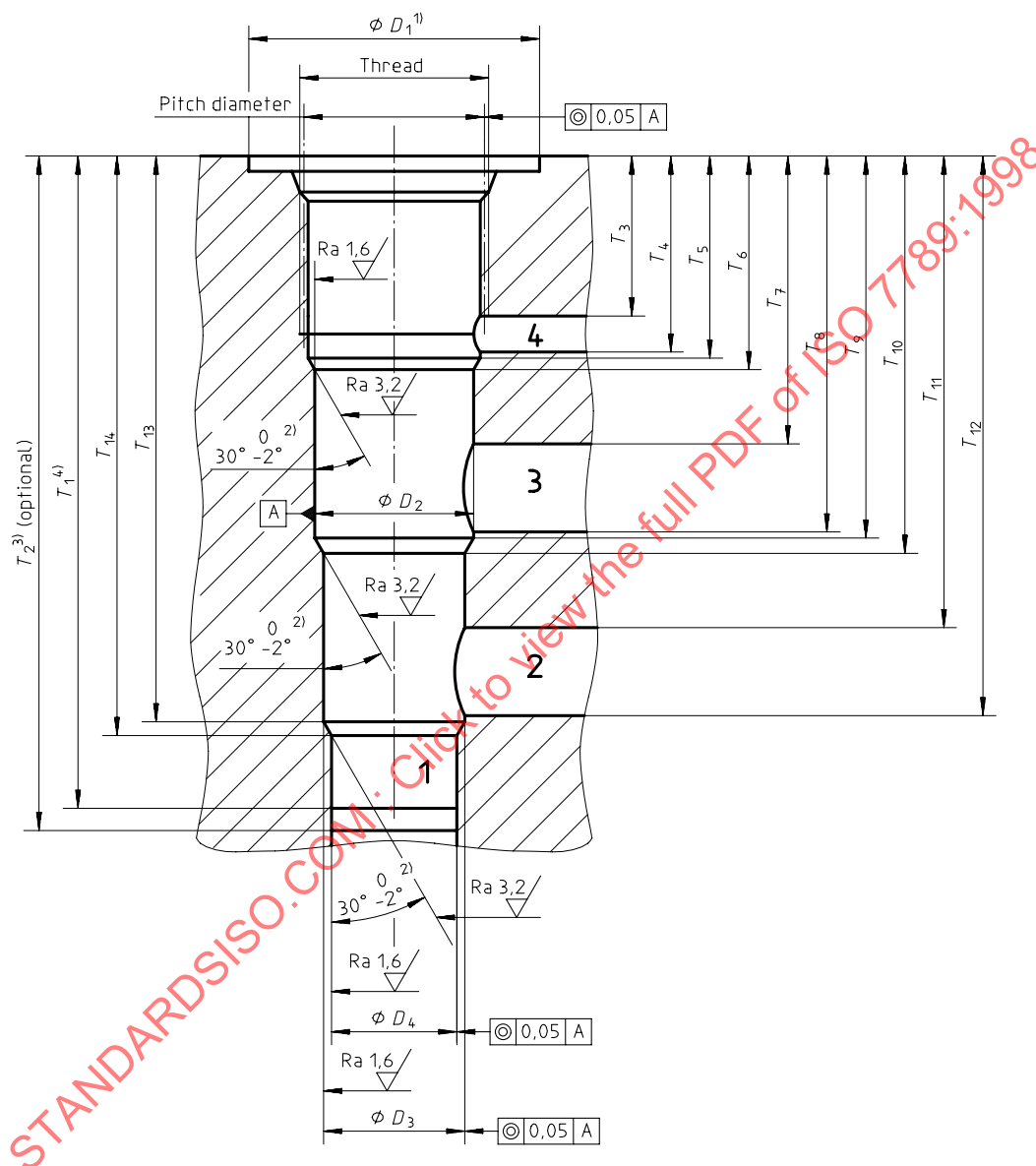
Figure 9 — Cavities for three-port valves with 10,5 mm to 20,5 mm maximum port diameter and one pilot port
