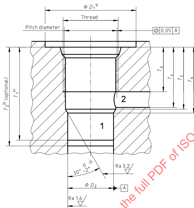
Figure 1 — Cavities for two-port valves (to excluding main system pressure relief valves) with 5 mm to 20,5 mm maximum port diameter
